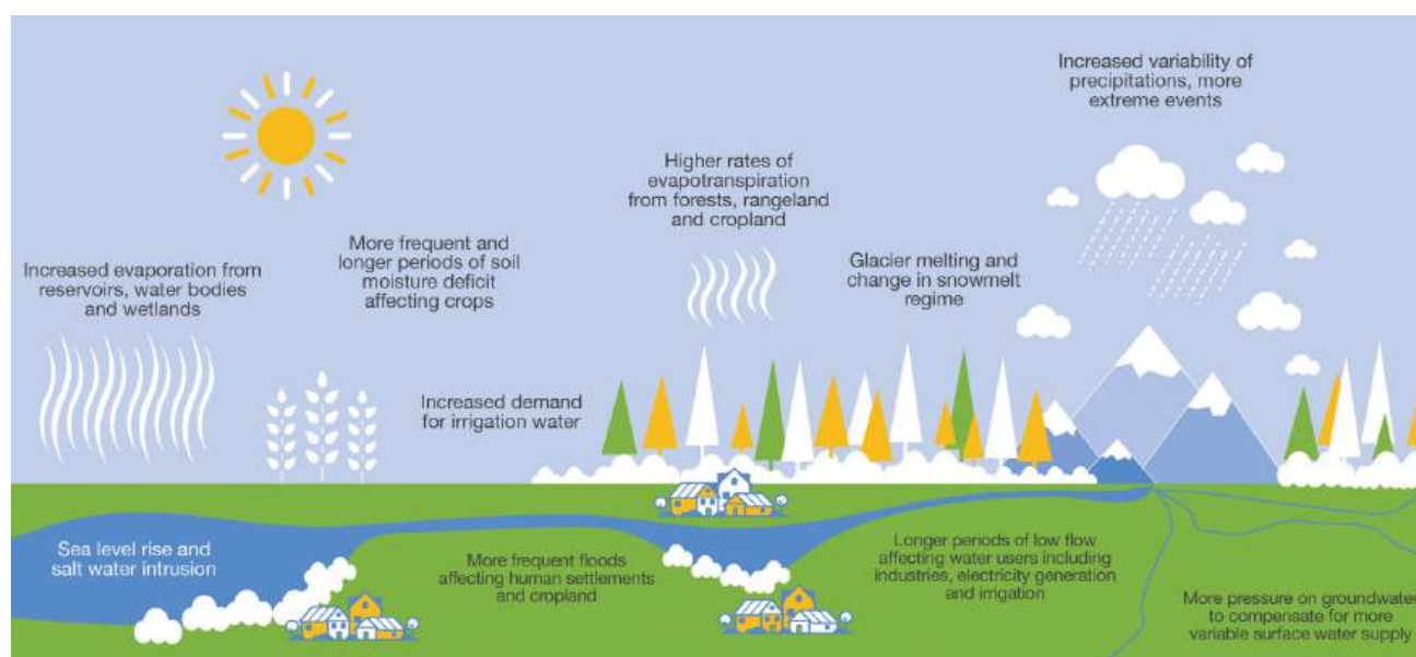
Figure 20 Links between climate change, water cycle, and agriculture 144
